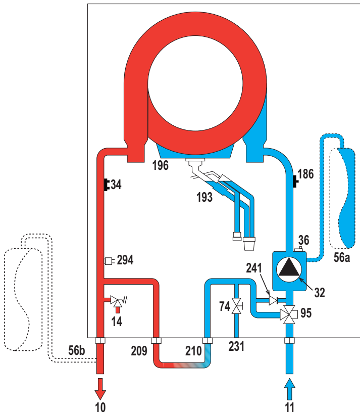
fig. 75- Hydraulic circuit
