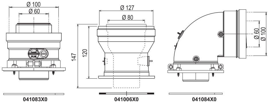
fig. 32- Starting accessories for coaxial ducts
