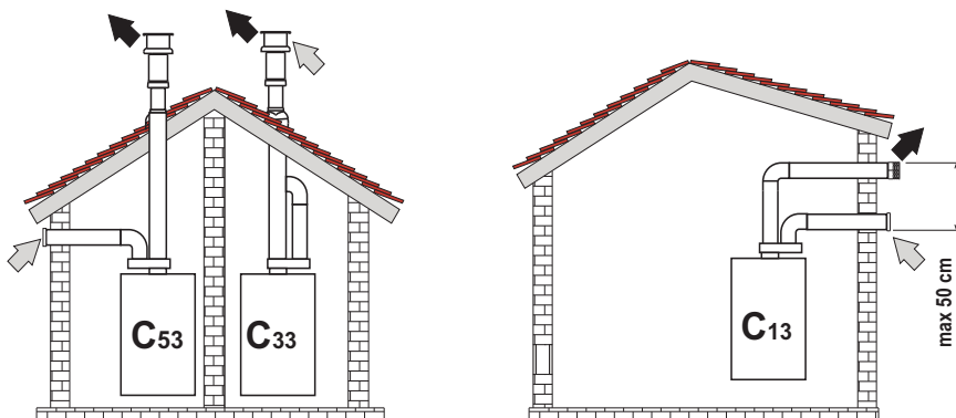
fig. 35- Examples of connection with separate pipes
